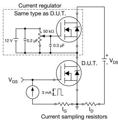
Fig. 19 - Gate Charge Test Circuit
