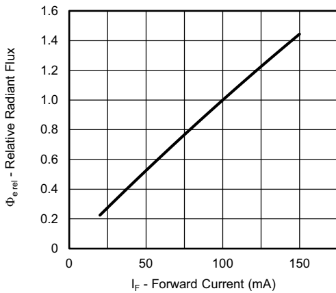
Fig. 2 - Relative Radiant Power vs. Forward Current
