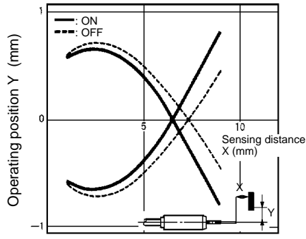
E3C-DM5/-DM5A (Typical)
