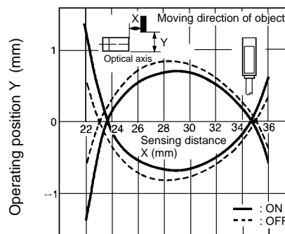
E3C-LS3R (Typical 1)
