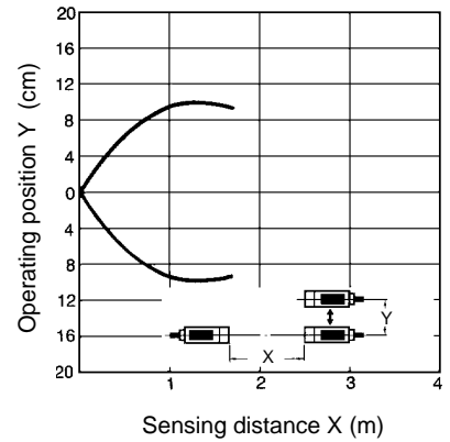
E3C-LS3R (Typical 2)
