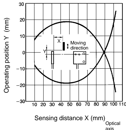
E3C-DS10 (Typical 2)
