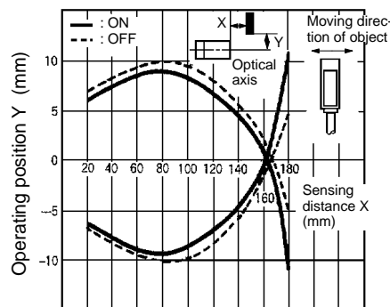
E3C-DS10 (Typical 2)
