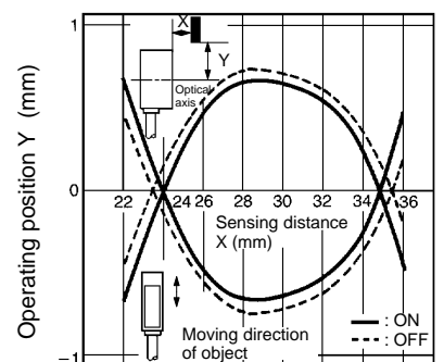
E3C-LS3R (Typical 2)
