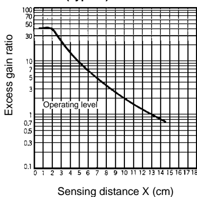
E3C-DS5W (Typical)
