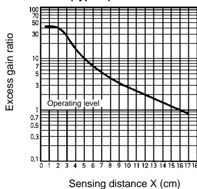
E3C-DS10T (Typical)
