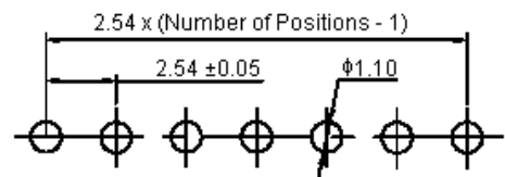
PCB Layout
