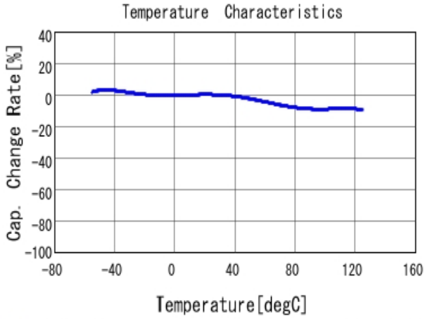
■ GCJ188R71C473KA01 C-Temp. capchange, DCO. 0V, AC1.0V r m
