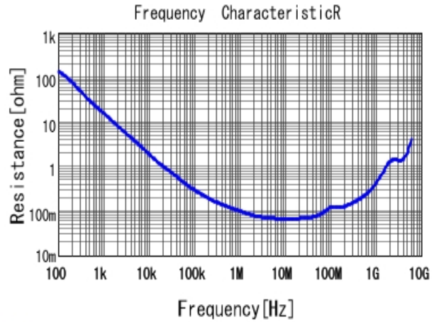
■ GCJ188R71C473KA01 R DCOV, 25degC
