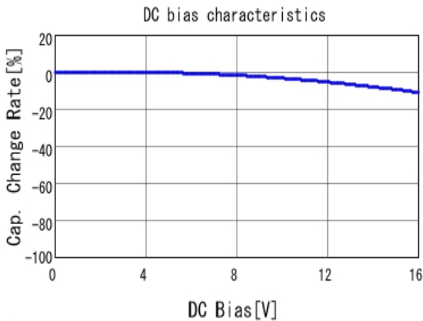
■ GCJ188R71C473KA01 C-DC bias capchange, 25.0degC, AC1.
