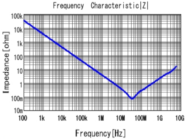
■ GCJ188R71C473KA01 |Z| DCOV, 25degC
