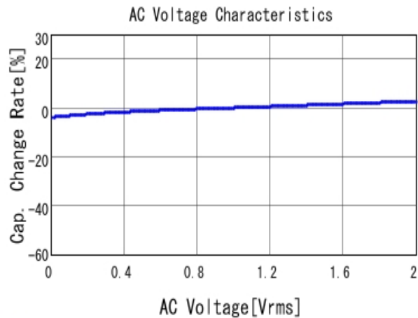
■ GCJ188R71C473KA01 C-AC Voltage capchange, DCOV, 25.0d
