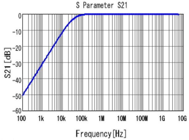
■ GCJ188R71C473KA01 S21 DCOV, 25degC
