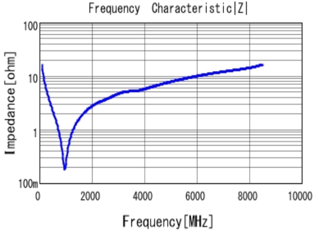
■ GCM0335C1H101FA16 |Z| DC0V, 25degC
