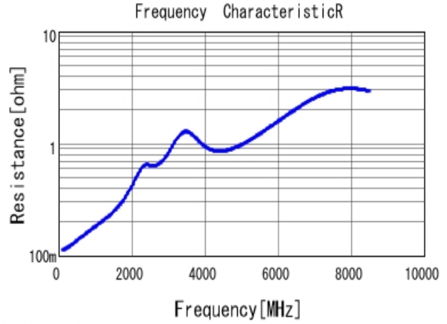
■ GCM0335C1H101FA16 R DC0V, 25degC
