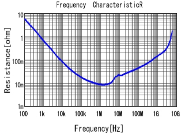
■ GRJ188C70J475KE11 R DCOV, 25degC
