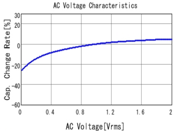
■ GRJ188C70J475KE11 C-AC Voltage capchange, DCOV, 25.0d
