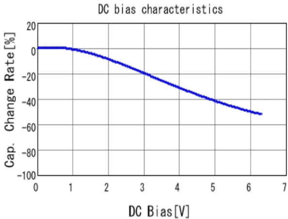
■ GRJ188C70J475KE11 C-DC bias capchange, 25.0degC, AC1V
