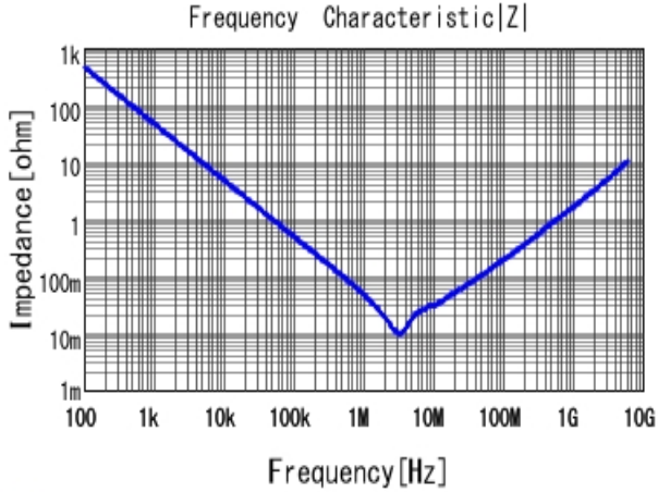
■ GRJ188C70J475KE11 |Z| DCOV, 25degC
