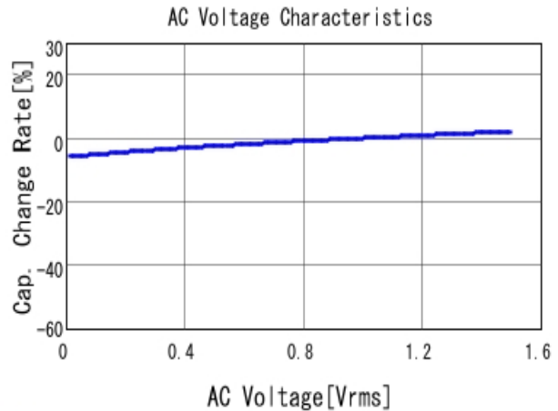
■ GRM32EC72A106KE05 C-AC Voltage capchange, DCOV, 25.0d
