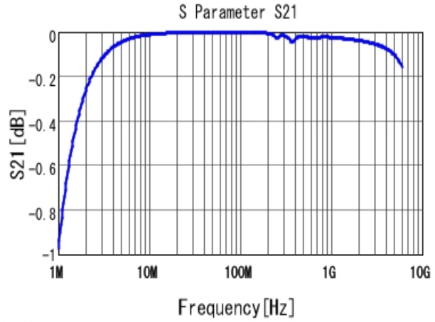
■ GRM1885C2A332JA01 S21 DCOV, 25degC
