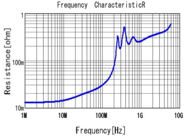
■ GRM1885C2A332JA01 R DCOV, 25degC
