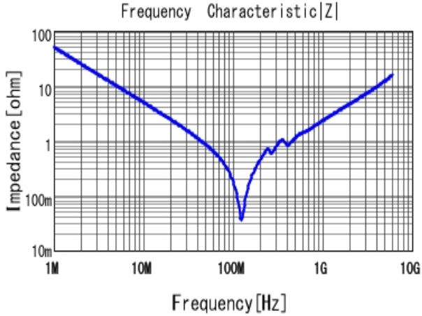
■ GRM1885C2A332JA01 |Z| DCOV, 25degC
