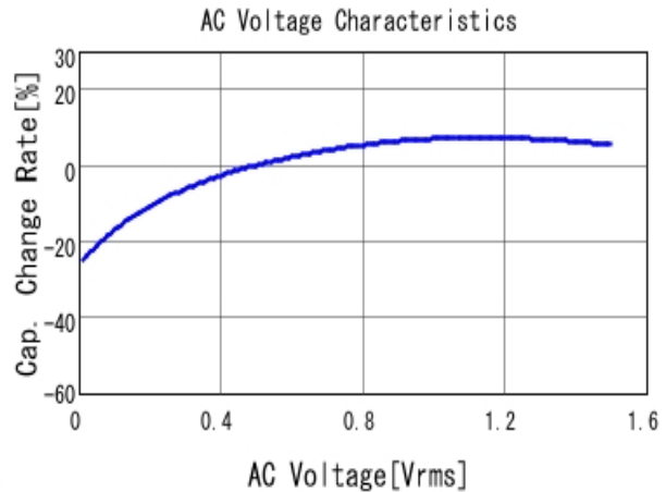
■ GRM188B31A106ME69 C-AC Voltage capchange, DCOV, 20.0d
