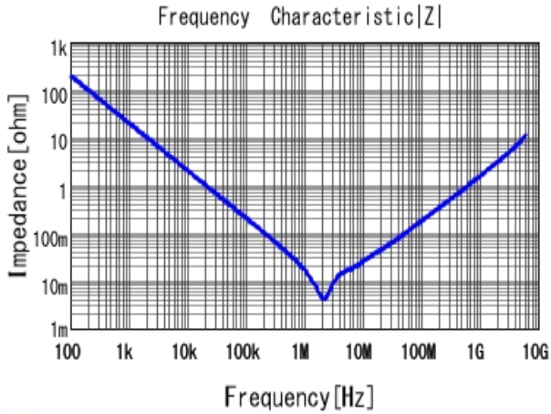
■ GRM188B31A106ME69 |Z| DCOV, 20degC
