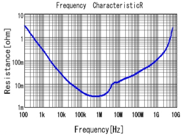
■ GRM188B31A106ME69 R DCOV, 20degC
