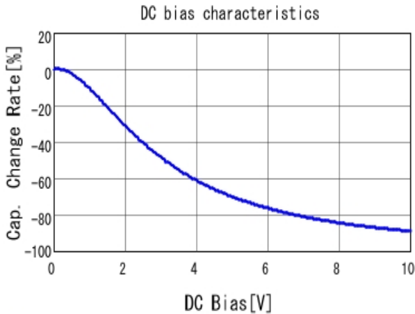
■ GRM188B31A106ME69 C-DC bias capchange, 20.0degC, AC0.
