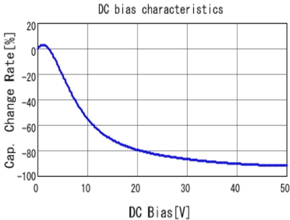
■ GRM319R61H475KA12 C-DC bias capchange, 25.0degC, AC1.
