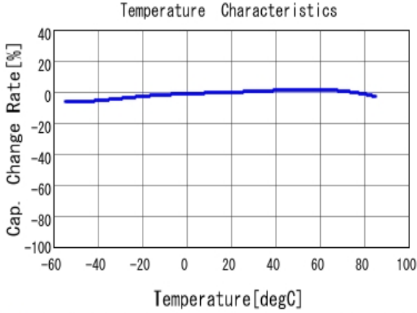
■ GRM319R61H475KA12 C-Temp. capchange, DC0.0V, AC1.0V rm
