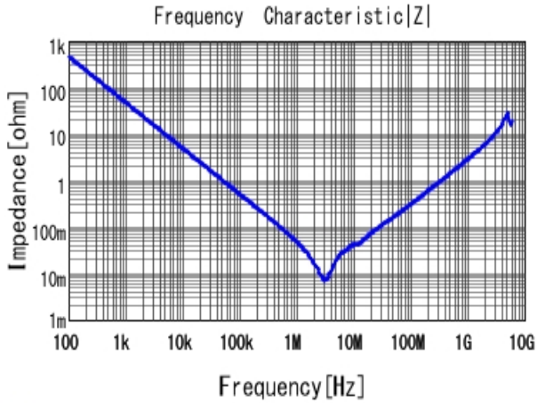
■ GRM319R61H475KA12 |Z| DCOV, 25degC
