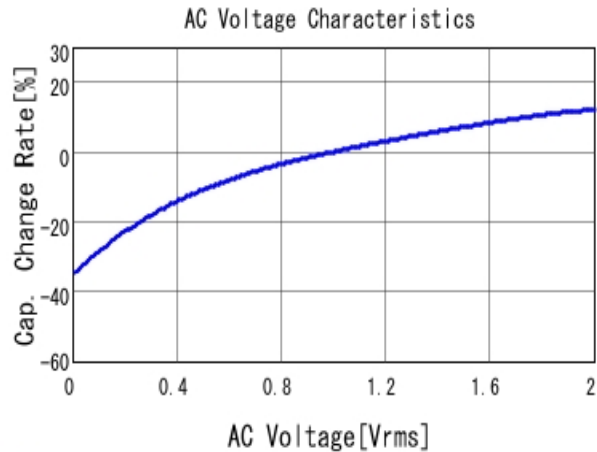
■ GRM319R61H475KA12 C-AC Voltage capchange, DCOV, 25.0d
