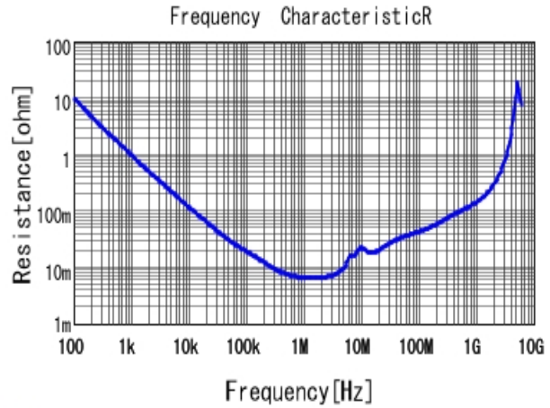
■ GRM319R61H475KA12 R DCOV, 25degC
