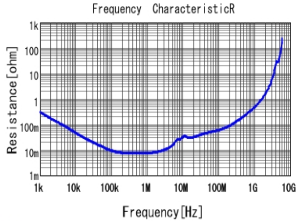
■ KRM31KR72A225KH01 R DCOV, 25degC
