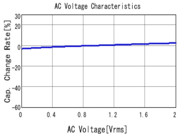
■ KRM31KR72A225KH01 C-AC Voltage capchange, DCOV, 25.0d
