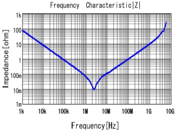
■ KRM31KR72A225KH01 |Z| DCOV, 25degC
