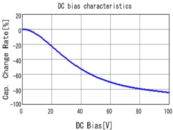
■ KRM31KR72A225KH01 C-DC bias capchange, 25.0degC, AC1V
