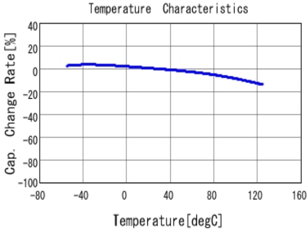
■ KRM31KR72A225KH01 C-Temp. capchange, DCOV, AC1Vrms
