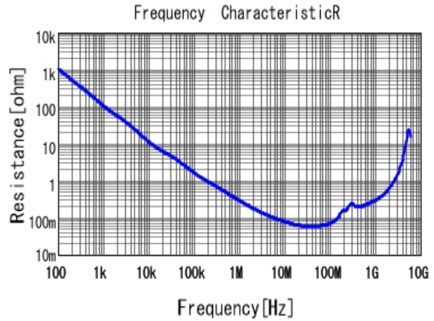
■ GCD188R71H682KA01 R DCOV, 25degC
