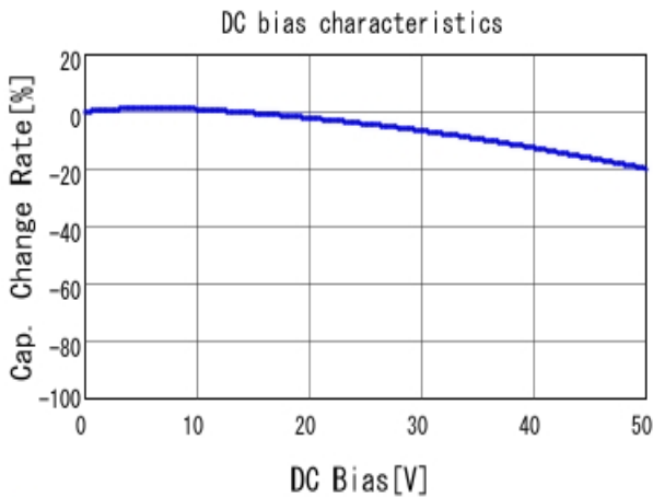
■ GCD188R71H682KA01 C-DC bias capchange, 25.0degC, AC1.
