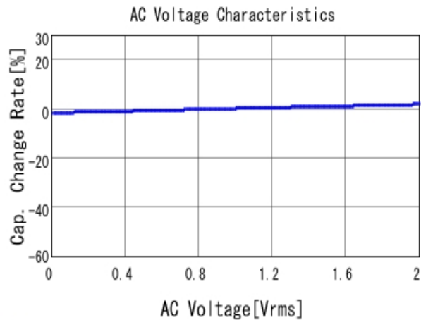
■ GCD188R71H682KA01 C-AC Voltage capchange, DCOV, 25.0d
