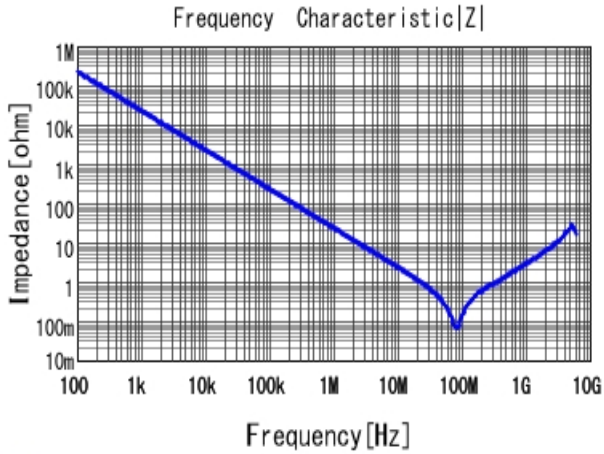
■ GCD188R71H682KA01 |Z| DCOV, 25degC
