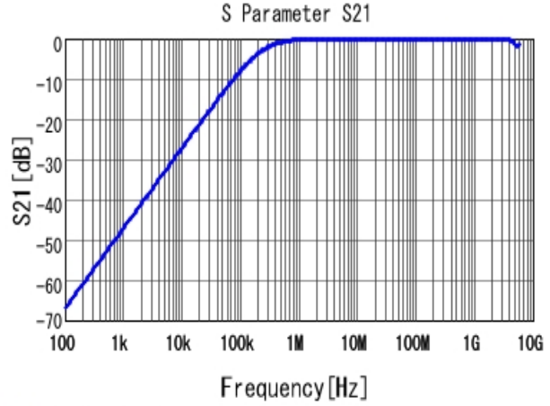
■ GCD188R71H682KA01 S21 DCOV, 25degC
