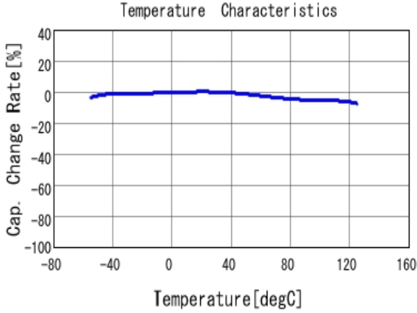
■ GCD188R71H682KA01 C-Temp. capchange, DCO. 0V, AC1.0V r m
