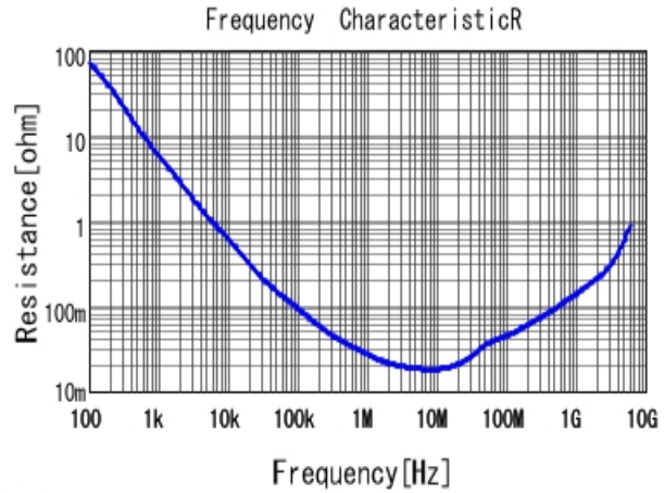
■ GRM033C80J224KE90 R DCOV, 25degC
