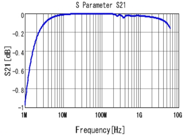
■ GRM1885C2A332JA01 S21 DCOV, 25degC
