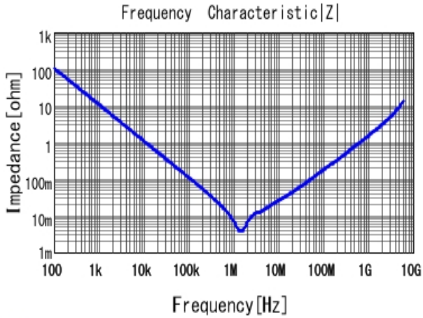
■ GRM188B30J226MEA0 |Z| DCOV, 20degC
