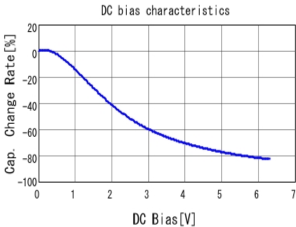
■ GRM188B30J226MEA0 C-DC bias capchange, 20.0degC, AC0.
