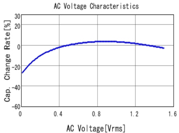
■ GRM188B30J226MEA0 C-AC Voltage capchange, DCOV, 20.0d
