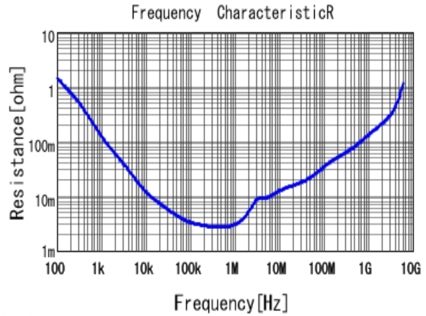
■ GRM188B30J226MEA0 R DCOV, 20degC
