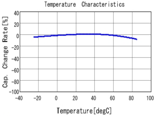
■ GRM188B31C475KAAJ C-Temp. capchange, DCO. 0V, ACO. 2V rm
