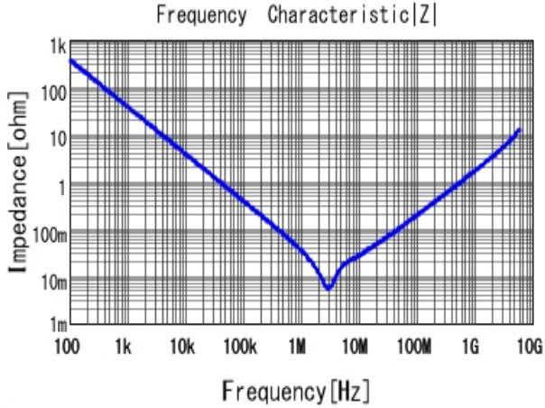
■ GRM188B31C475KAAJ |Z| DCOV, 20degC
