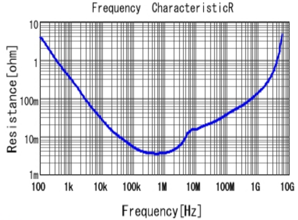
■ GRM188B31C475KAAJ R DCOV, 20degC
