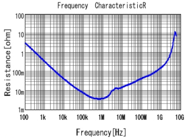
■ GRM319R61C226ME15 R DCOV, 25degC
