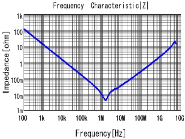
■ GRM319R61C226ME15 |Z| DCOV, 25degC
