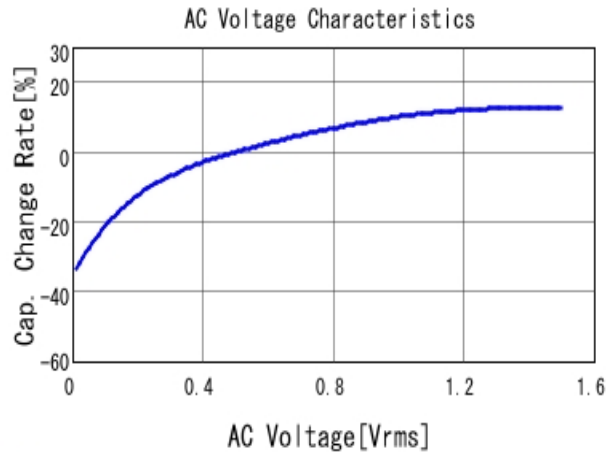
■ GRM319R61C226ME15 C-AC Voltage capchange, DCOV, 25.0d
