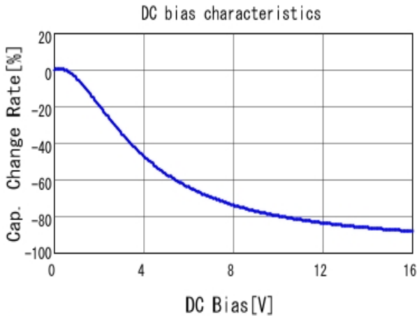
■ GRM319R61C226ME15 C-DC bias capchange, 25.0degC, AC0.
