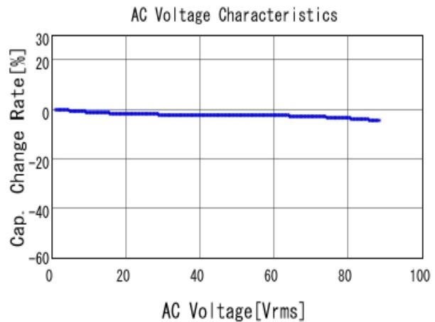
■ KRM55TR72E225MH01 C-AC Voltage capchange, DCOV, 25.0d
