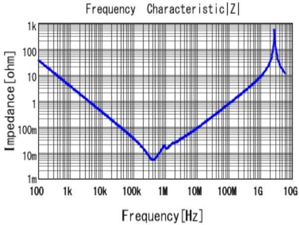
■ KRM55WR71E476MH01 |Z| DCOV, 25degC
