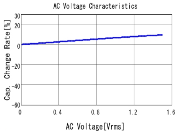
■ KRM55WR71E476MH01 C-AC Voltage capchange, DCOV, 25.0d
