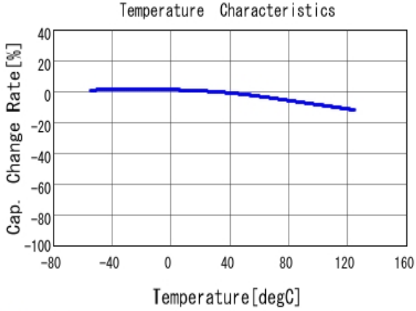
■ KRM55WR71E476MH01 C-Temp. capchange, DCOV, ACO, 5Vrms
