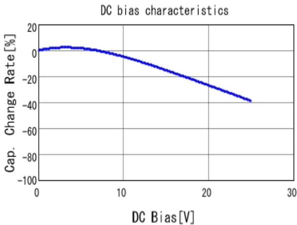
■ KRM55WR71E476MH01 C-DC bias capchange, 25.0degC, AC0.
