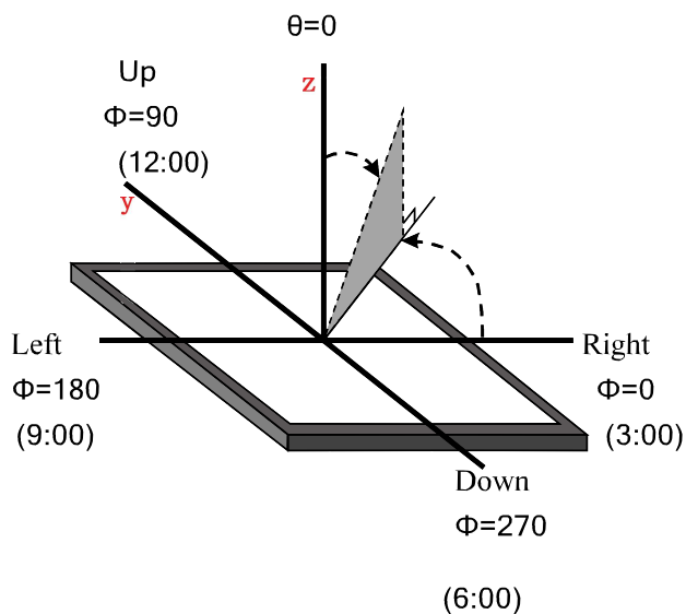
FIG.3.The definition of viewing angle
