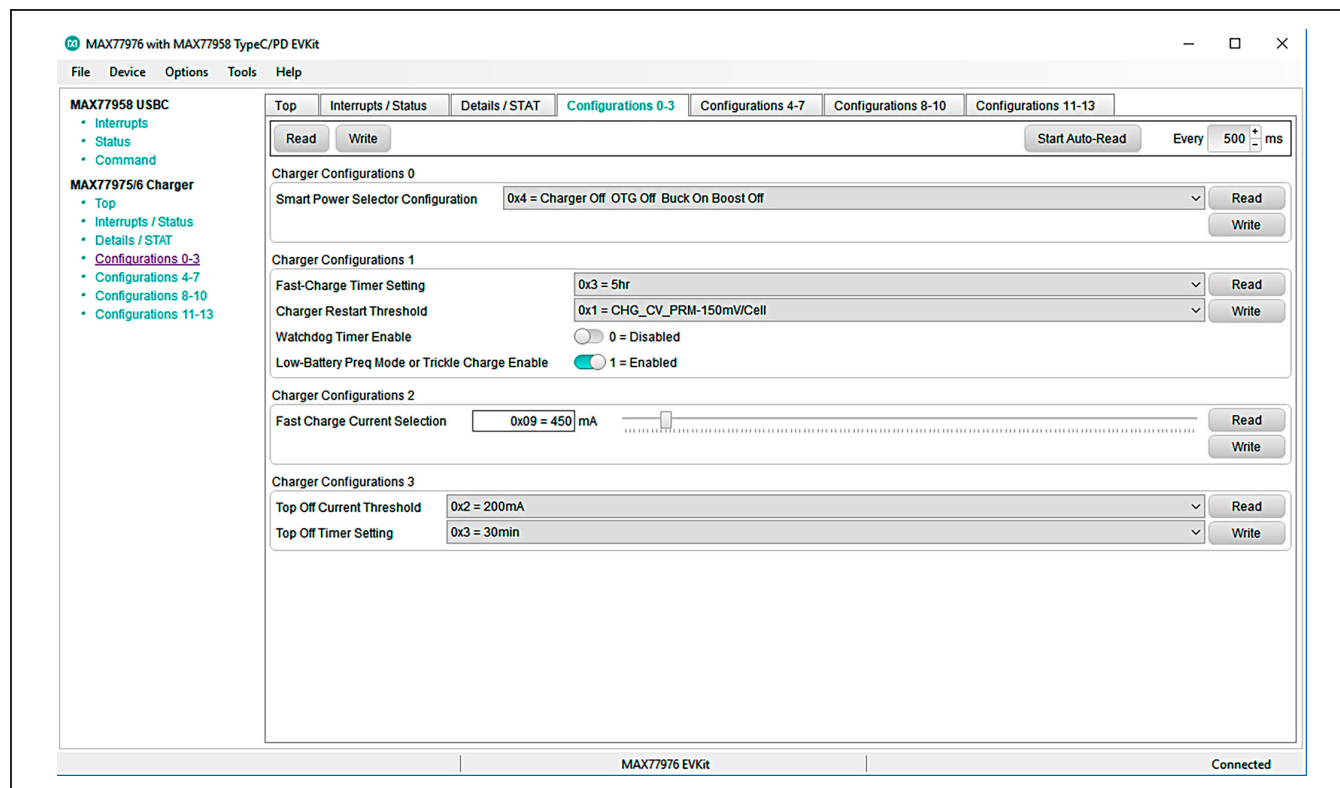
Figure 6. MAX77975/MAX77976 Configurations
