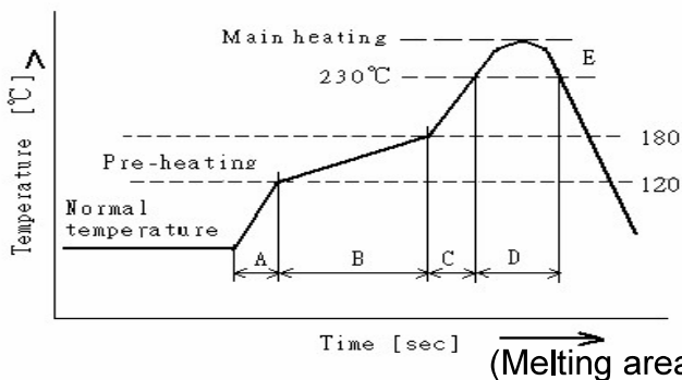
Temperature Profile
