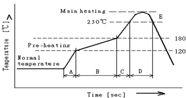
Temperature Profile
