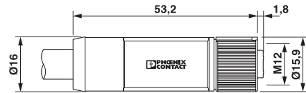
M12 x 1 socket, straight
