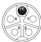
Pin assignment of M12 socket, 5-pos., K-coded, socket side view
