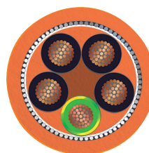
PUR halogen-free orange [PUR]
