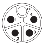
Pin assignment of M12 connector, 5-pos., L-coded, pin side view
