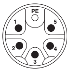
Pin assignment of M12 connector, 6-pos., M-coded, pin side view
