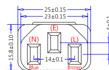
FM-302LSR (IEC 60320, C13, 15A 125V~) (Dimensions of Connector Face)
