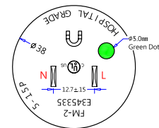
FM-2 (NEMA 5-15P, Hospital Grade) (Dimensions of Plug Face)
