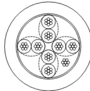
Cable Diagram
