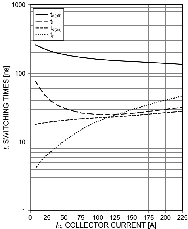
Figure 7. Typical switching times as a function of collector current (inductive load, T_{vj}=150^{\circ}C , V_{CE}=400V , V_{GE}=15/0V , R_G=5.6\Omega , Dynamic test circuit in Figure E)
