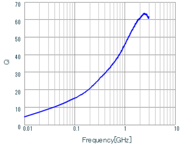
LQG15WZ4N1S02 Q.
