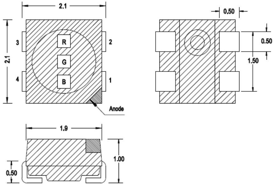
Figure 1: Package Drawing
