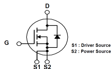
N-Channel MOSFET
