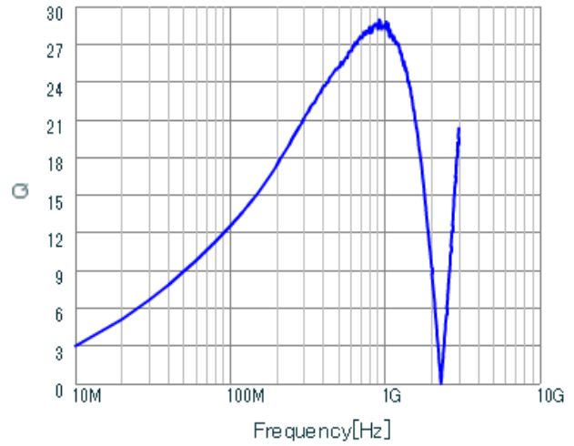
LQP03HQ43NJ02 Q.
