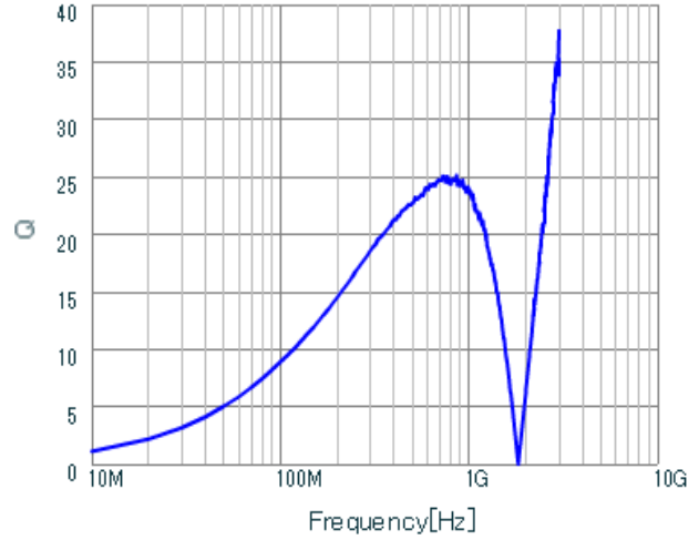
LQP03HQ75NJ02 Q.
