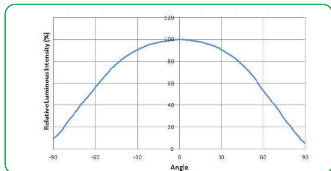
Radiation of a single LED - Beam Angle 125°
