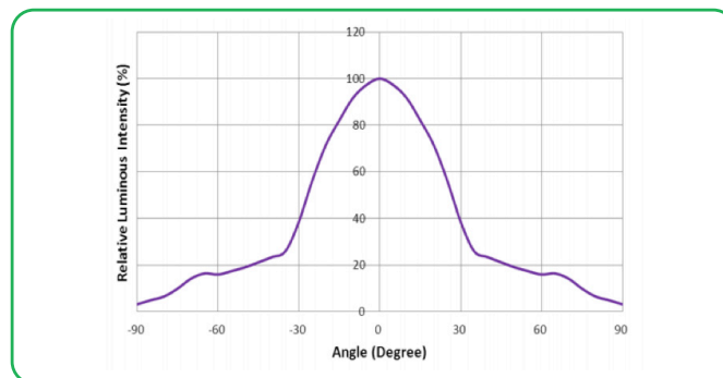
Radiation of a single LED - Beam Angle 55°
