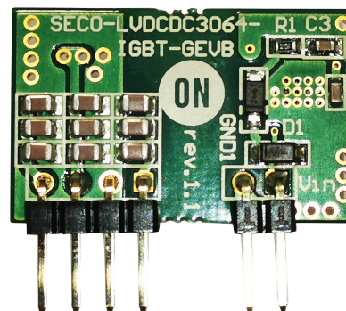
Figure 1. Board Layout
