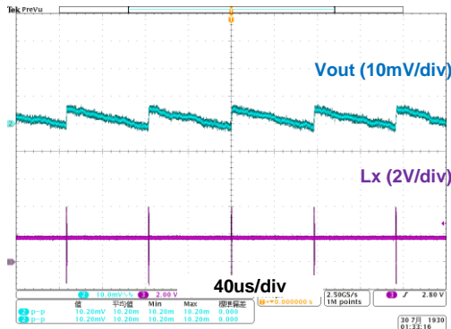
(4-1) Vin = 3.6V, Iout = 1mA
