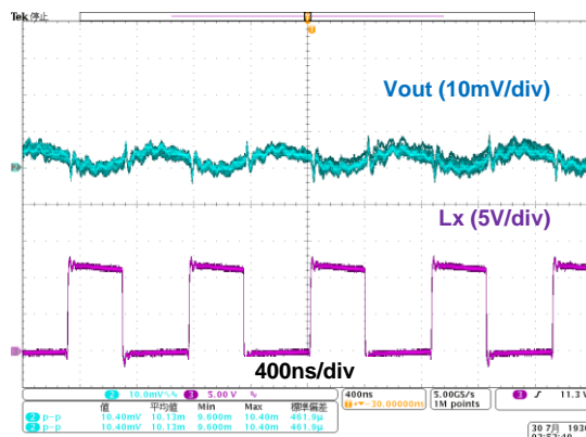
(4-2) Vin = 12V, Iout = 300mA
