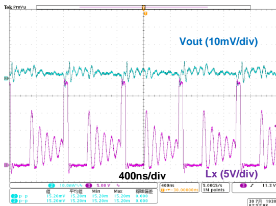
(4-3) Vin = 24V, Iout = 50mA
