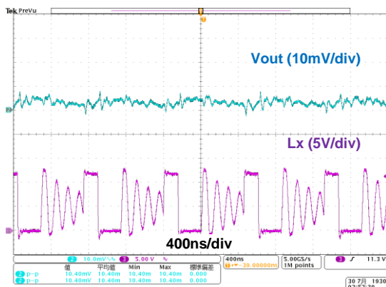
(4-1) Vin = 12V, Iout = 50mA
