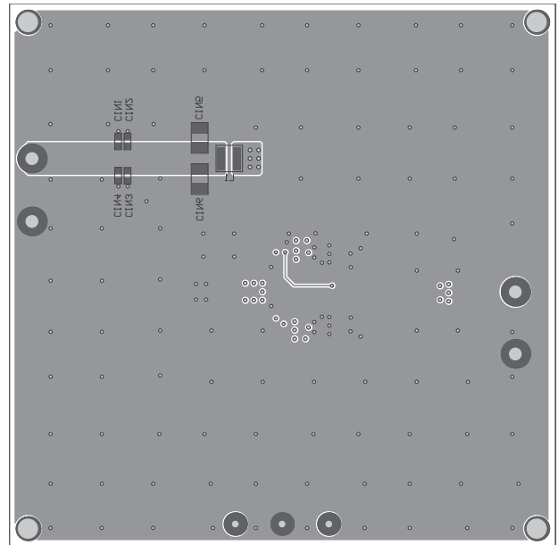
Figure 5: Bottom Layer and Bottom Silk
