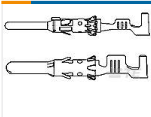
TE Part # 1703018-1 DIA 1.5MM CONTACT PIN,LP
