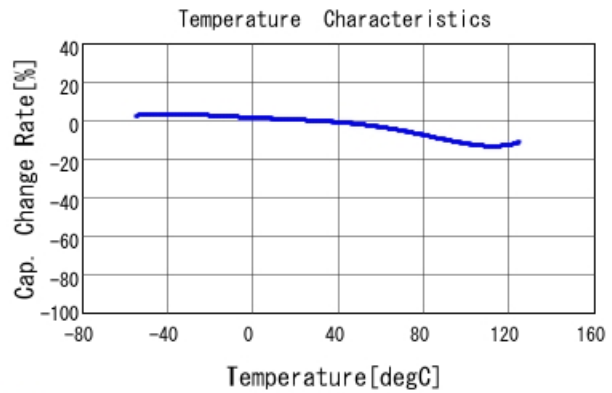
■ GR442QR73D152KW01 C-Temp. capchange, DCOV, AC1Vrms
