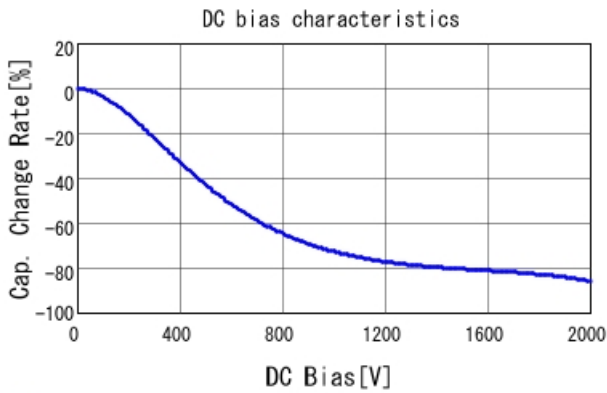
■ GR442QR73D152KW01 C-DC bias capchange, 25.0degC, AC1V
