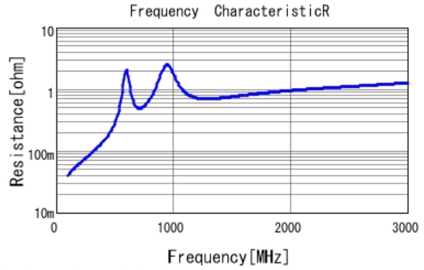
■ GRM31A5C3A471JWA1 R DCOV, 25degC
