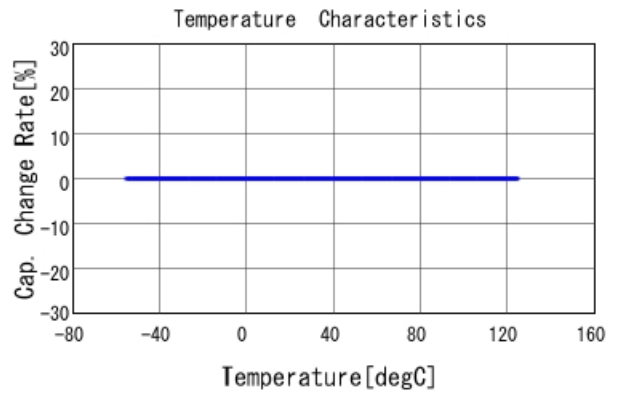
■ GRM31A5C3A471JWA1 C-Temp. capchange, DCOV, AC1Vrms
