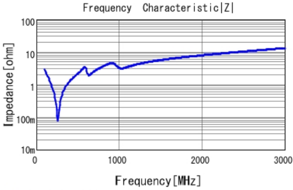
■ GRM31A5C3A471JWA1 |Z| DCOV, 25degC
