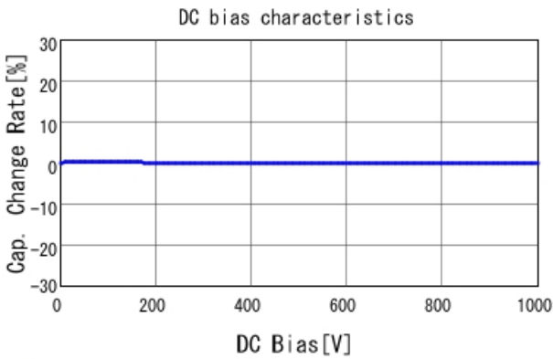
■ GRM31A5C3A471JWA1 C-DC bias capchange, 25.0degC, AC1V
