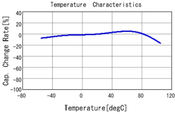
■ GRT31CC8YA106KE01 C-Temp. capchange, DCO. 0V, AC1. 0Vrm
