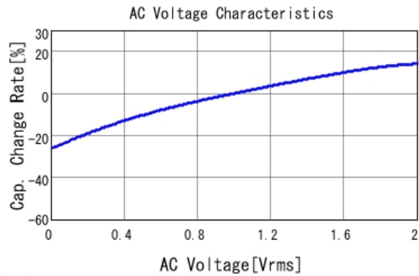
■ GRT31CC8YA106KE01 C-AC Voltage capchange, DCOV, 25.0d
