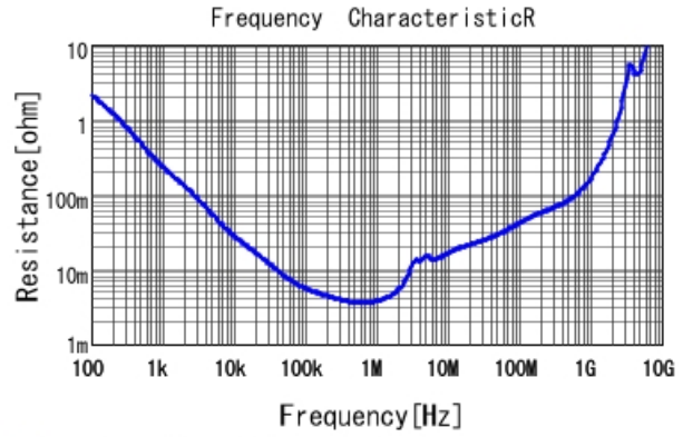
■ GRT31CC8YA106KE01 R DCOV, 25degC
