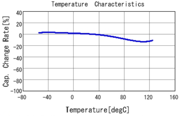
■ GA243QR7E2332MW01 C-Temp. capchange, DCOV, AC1Vrms
