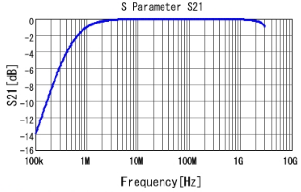
■ GA243QR7E2332MW01 S21 DCOV, 25degC
