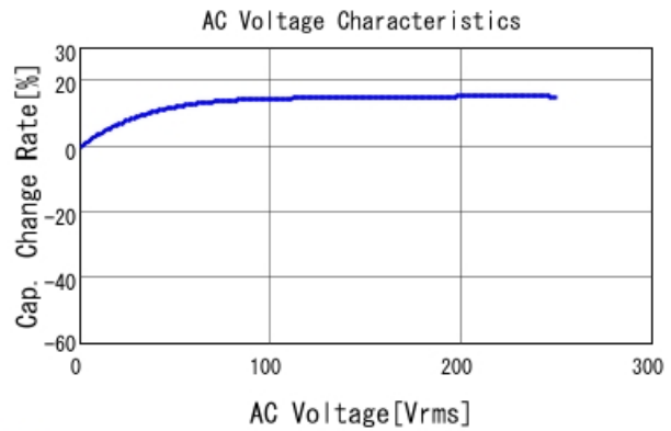
■ GA243QR7E2332MW01 C-AC Voltage capchange, DC0V, 25.0d
