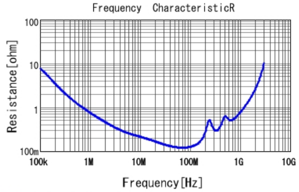
■ GA243QR7E2332MW01 R DC0V, 25degC
