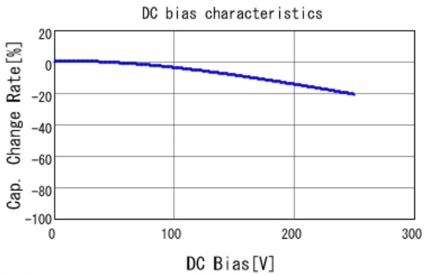
■ GA243QR7E2332MW01 C-DC bias capchange, 25.0degC, AC1V
