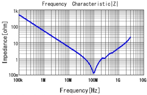
■ GA243QR7E2332MW01 |Z| DC0V, 25degC
