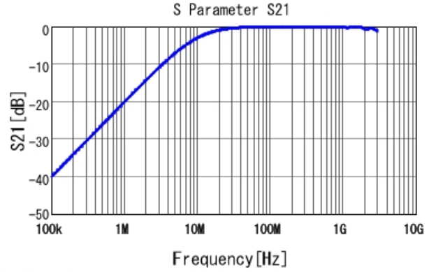
■ GA352QR7GF151KW31 S21 DCOV, 25degC
