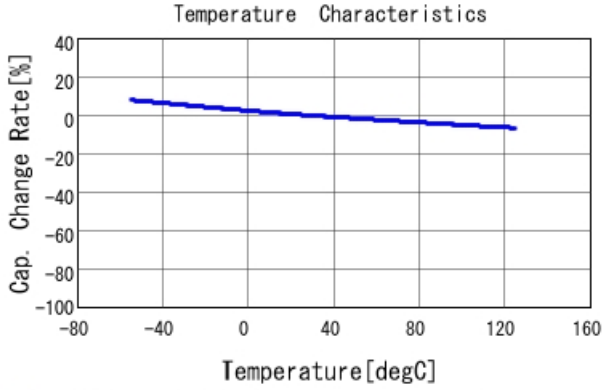
■ GA352QR7GF151KW31 C-Temp. capchange, DCOV, AC1Vrms
