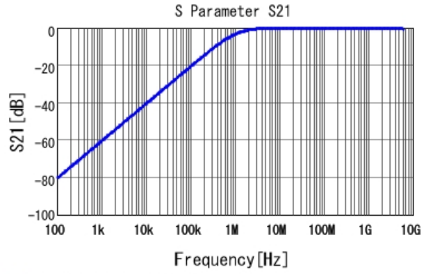
■ GCD188R71H152KA01 S21 DCOV, 25degC
