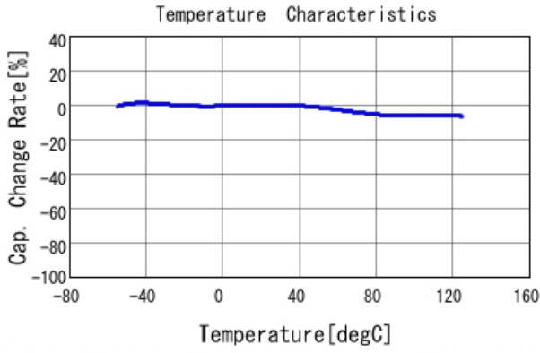
■ GCD188R71H152KA01 C-Temp. capchange, DCO. 0V, AC1. 0Vrm
